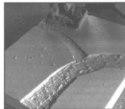
Finished channels
