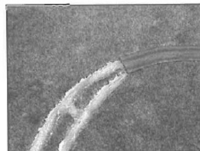
finished paths
